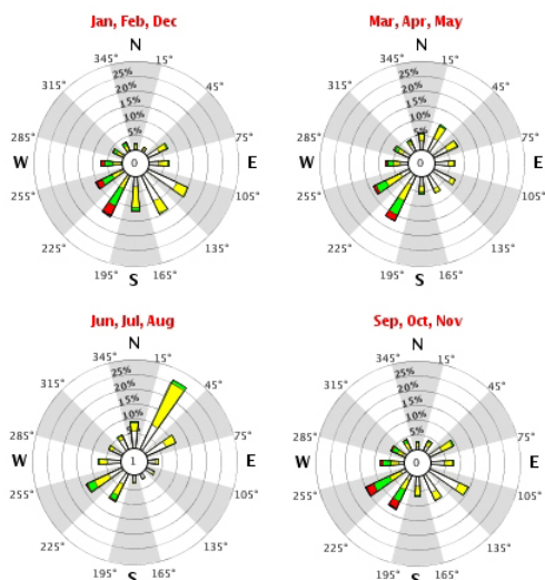
Wind rose, frequency distribution of wind
